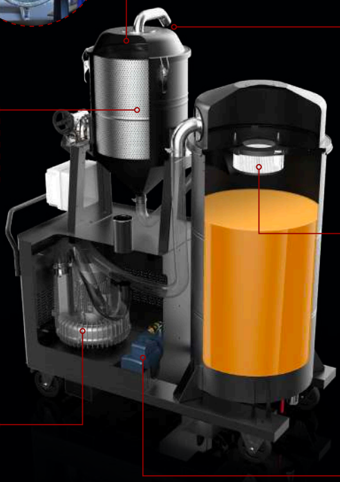
Discharge pump
