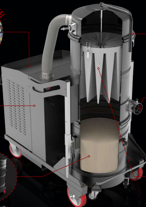
Kit HEPA filter (H14)
