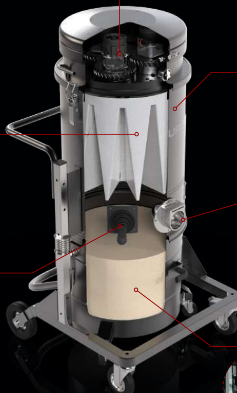
3 By-Pass motors
